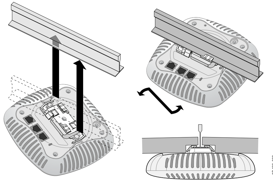
Figure 4 Mounting the AP
