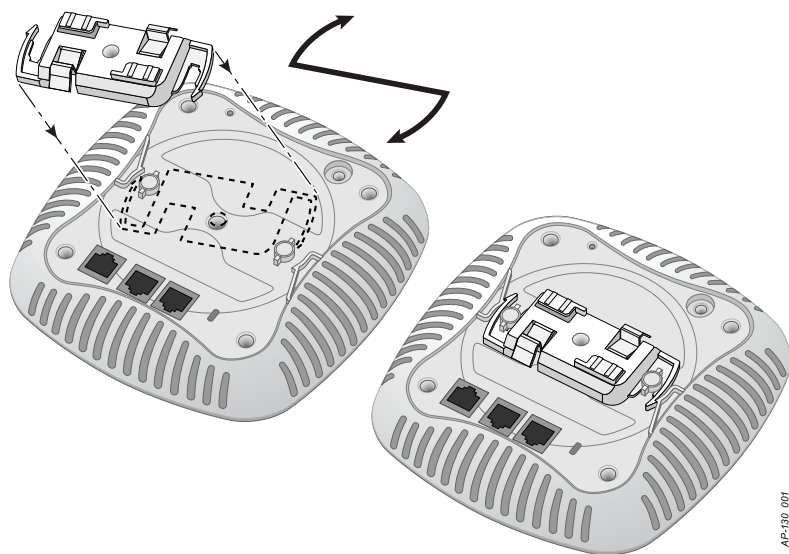
Figure 3 Attaching the Ceiling Rail Adapter
