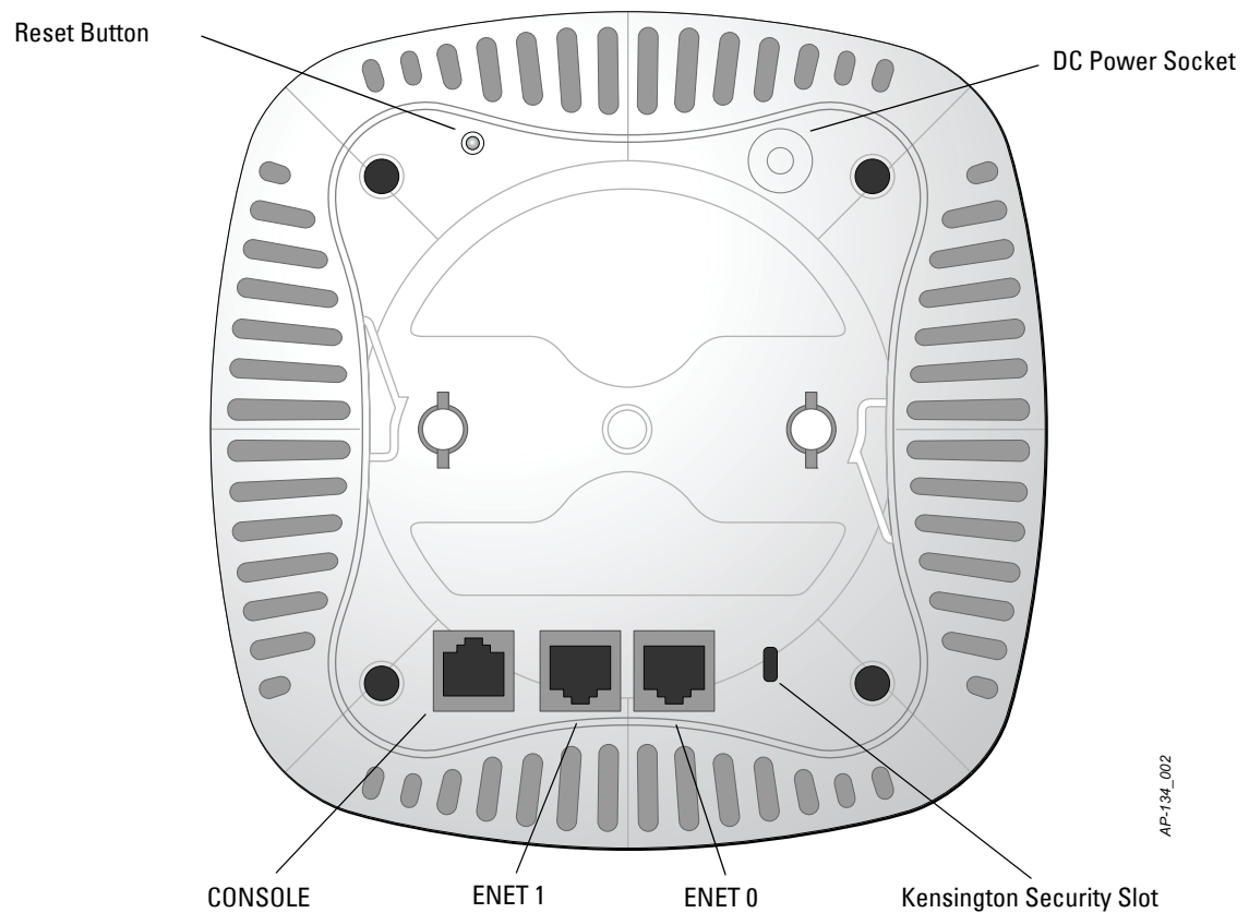
Figure 2 W-AP130 Series Rear
